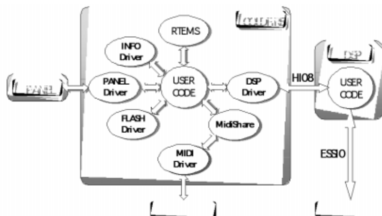
Figure 3: Software blocks of a full Chameleon application
