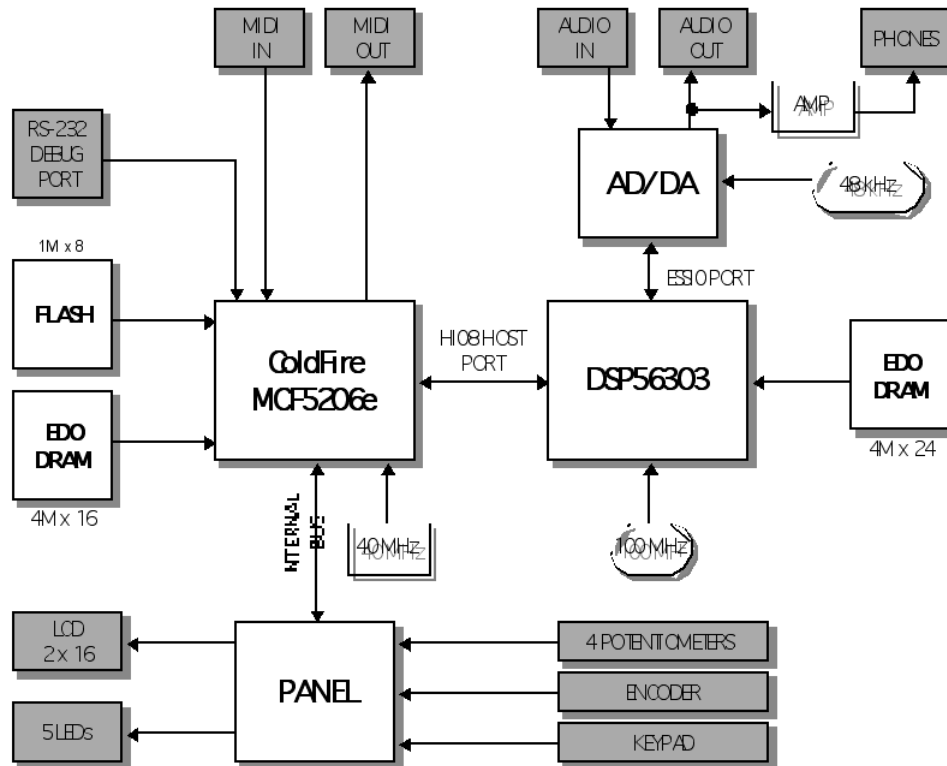
Figure 2: Chameleon architecture
